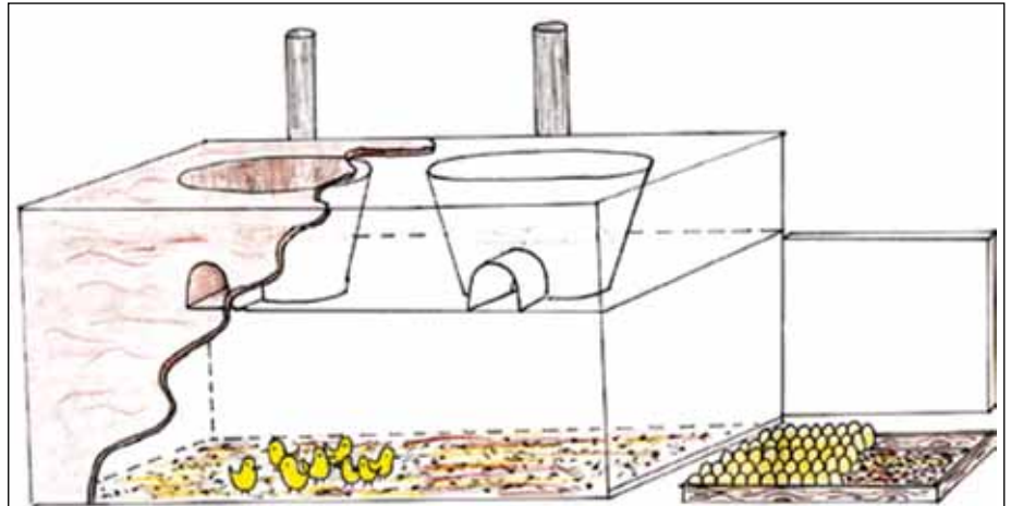
The incubator Ronald Nyagaka built looks like a common oven: The top with two fireplaces is used for cooking. Under these fireplaces is a chamber, the incubator, which retains the heat from the fireplace. The chamber has a door that can be closed overnight. In front of the door lies a tray with eggs. (Graphic by: S. Nganga)
